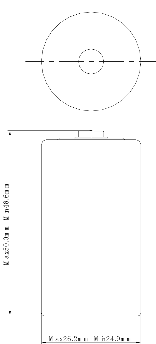
Battery Dimension R14P-Metal-702
