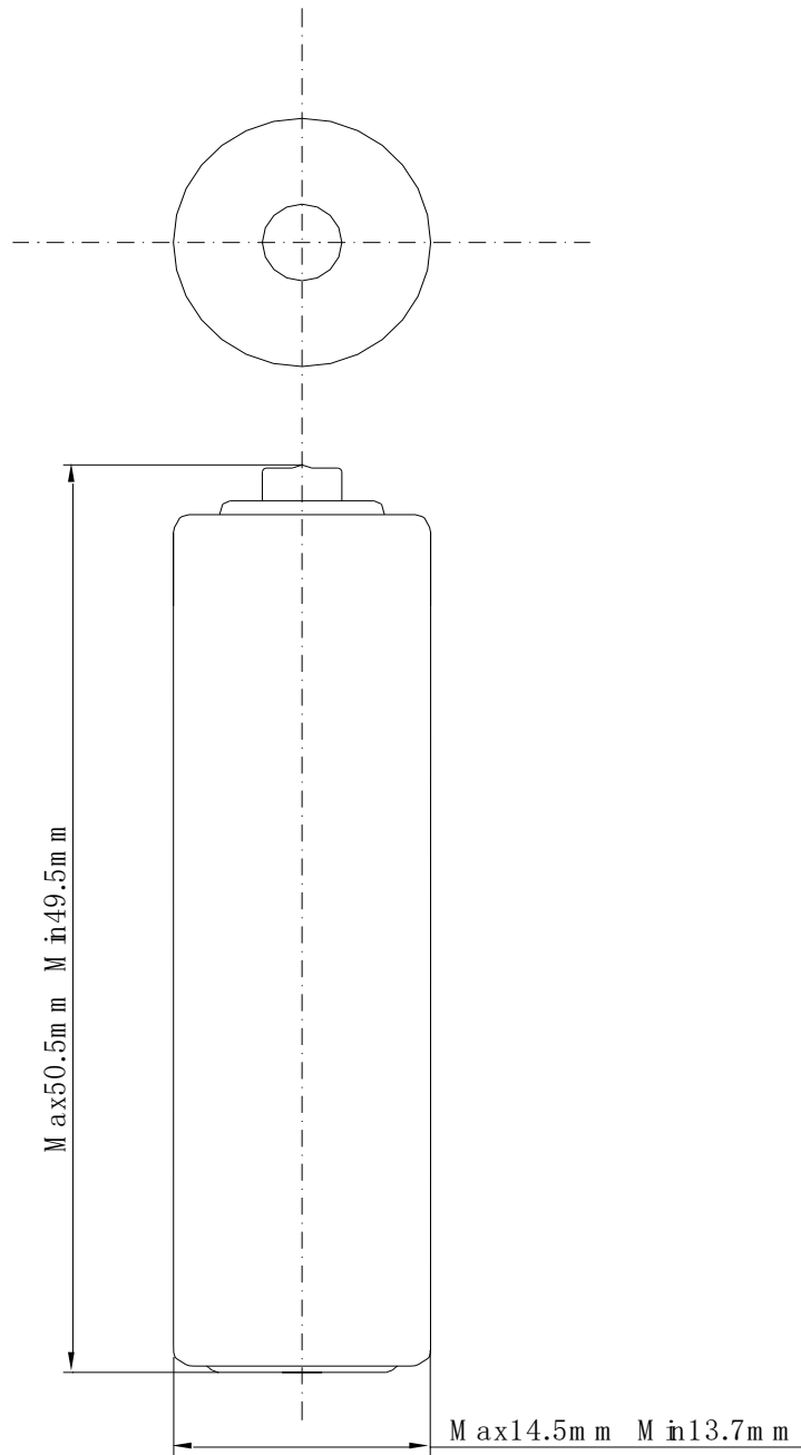
Battery Dimension R6P-Aluminum Foil-703
