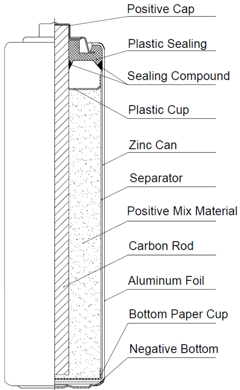
Battery Structure R6P-Aluminum Foil-703
