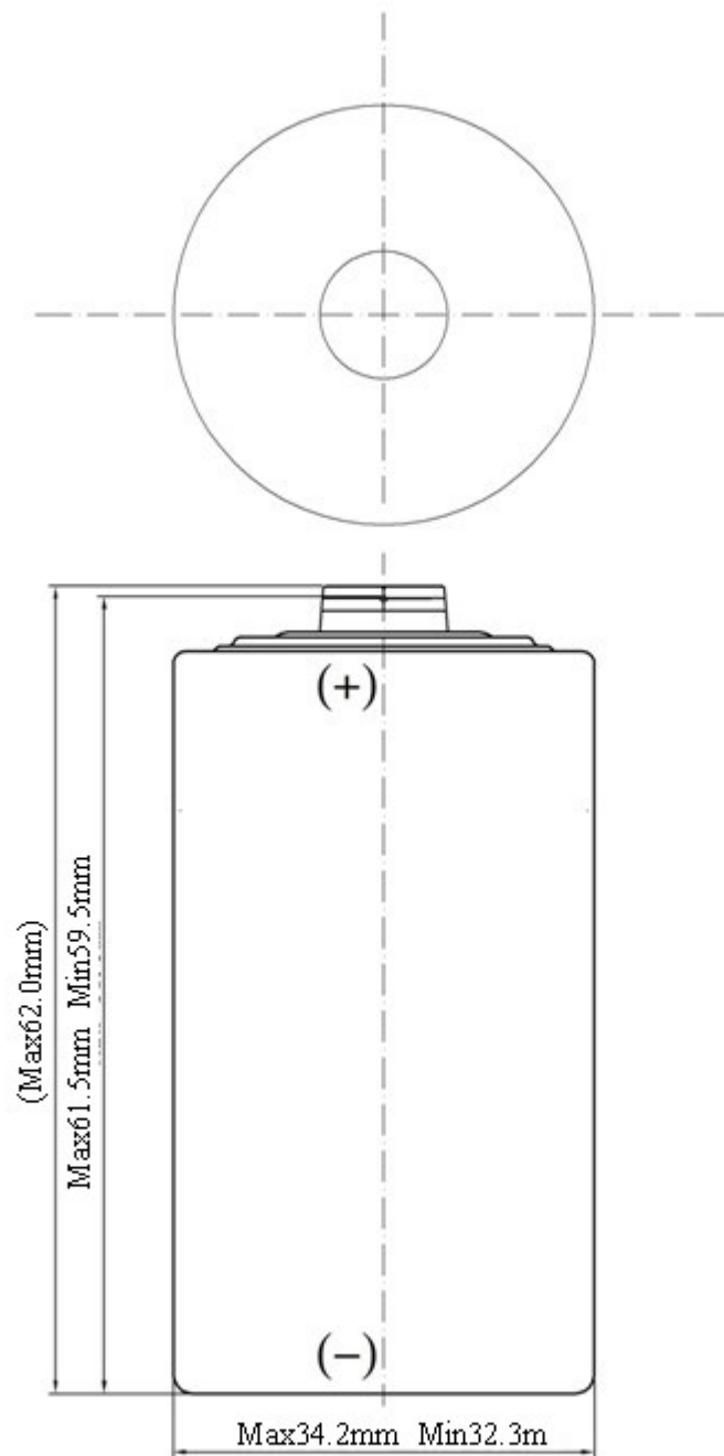
R20S-PVC-301A Battery Dimension
