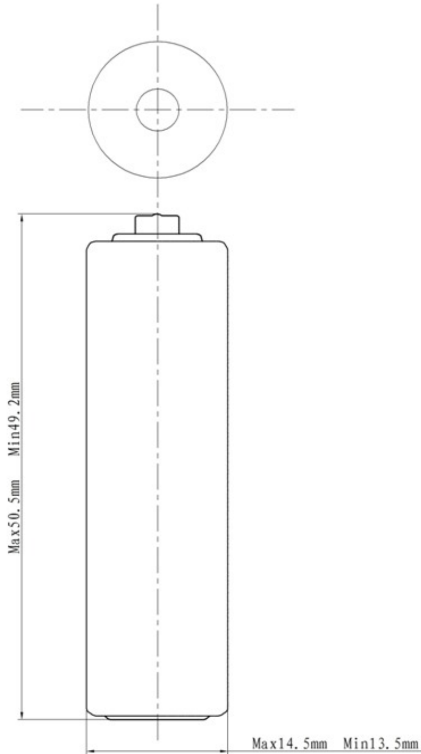
Battery Dimension R6P-PVC-303
